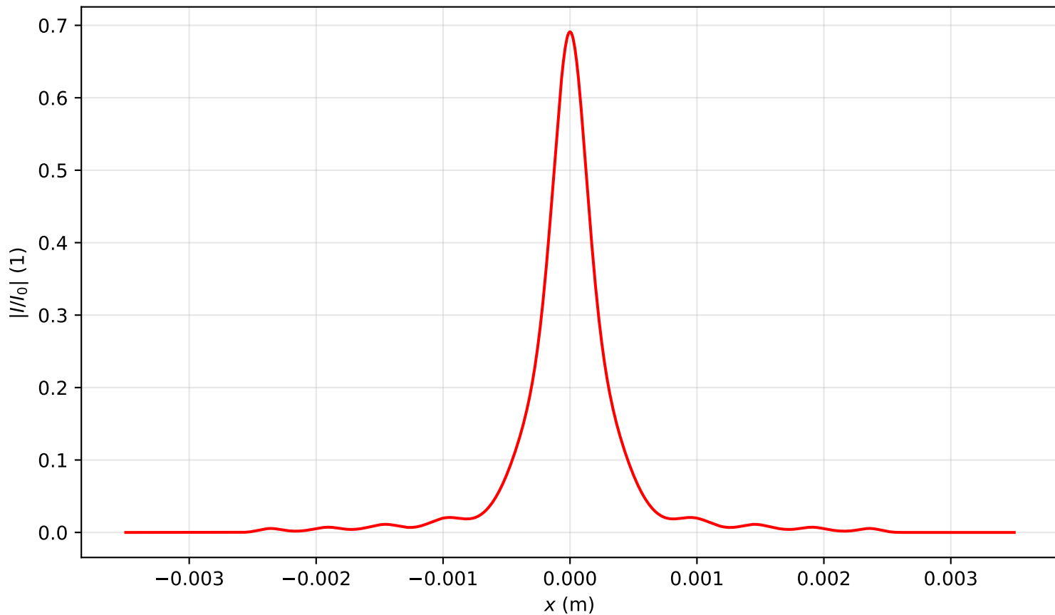
Intensity profile I(x, y = 0, z = 3.184)/I_0 , P_{in}=3.0P_{cr} , artificial time
